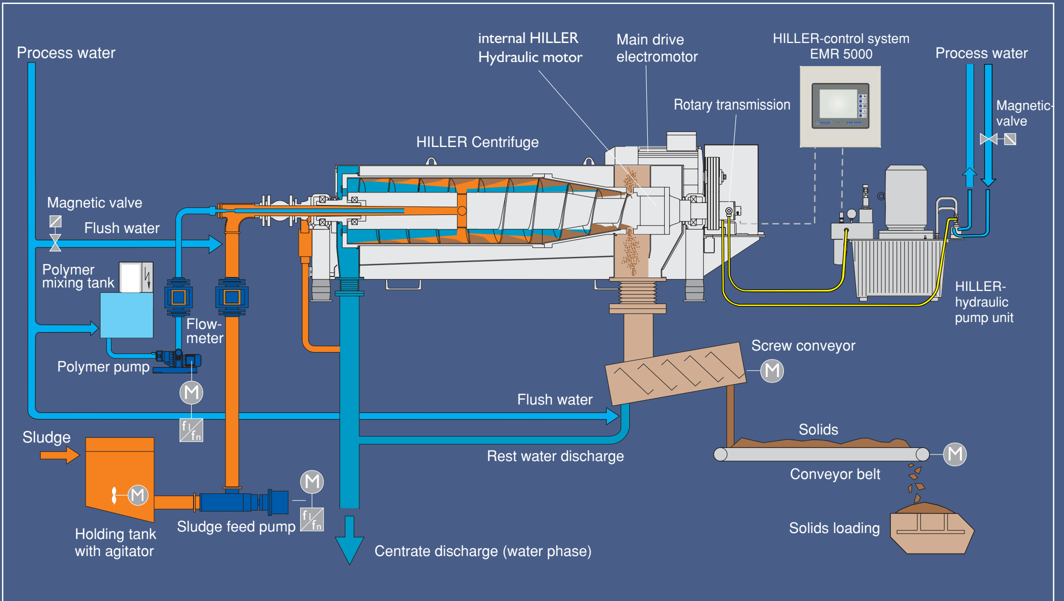
Schematic diagram with a HILLER-DecaPress® Centrifuge installation for dewatering of sewage sludge
